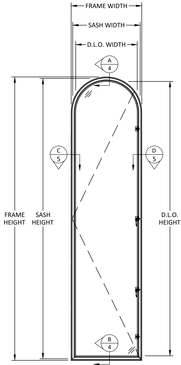
TYPICAL ELEVATION ROUND TOP
