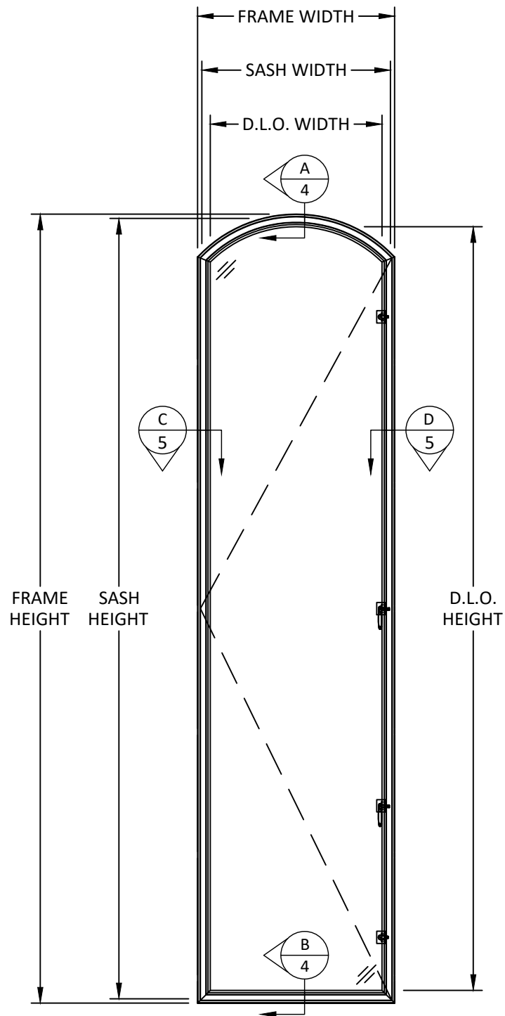
TYPICAL ELEVATION ARCH TOP
