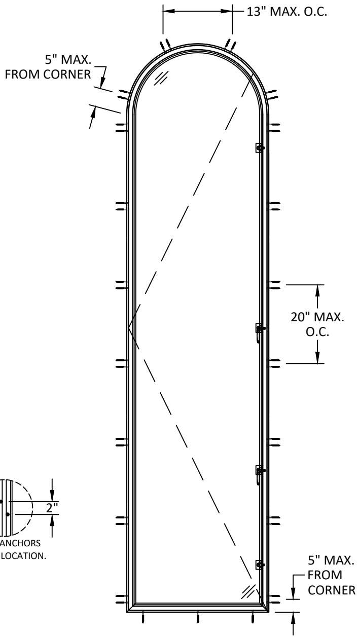
ANCHOR LAYOUT ROUND TOP
