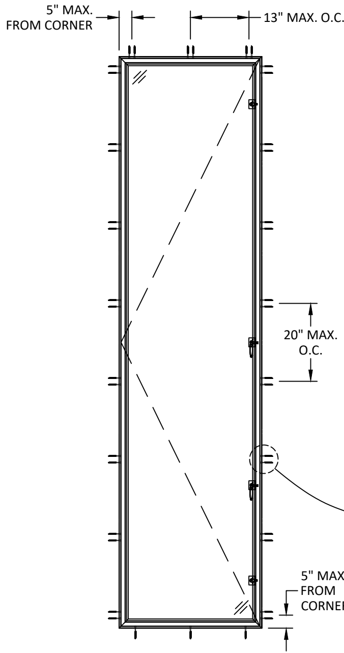
ANCHOR LAYOUT
