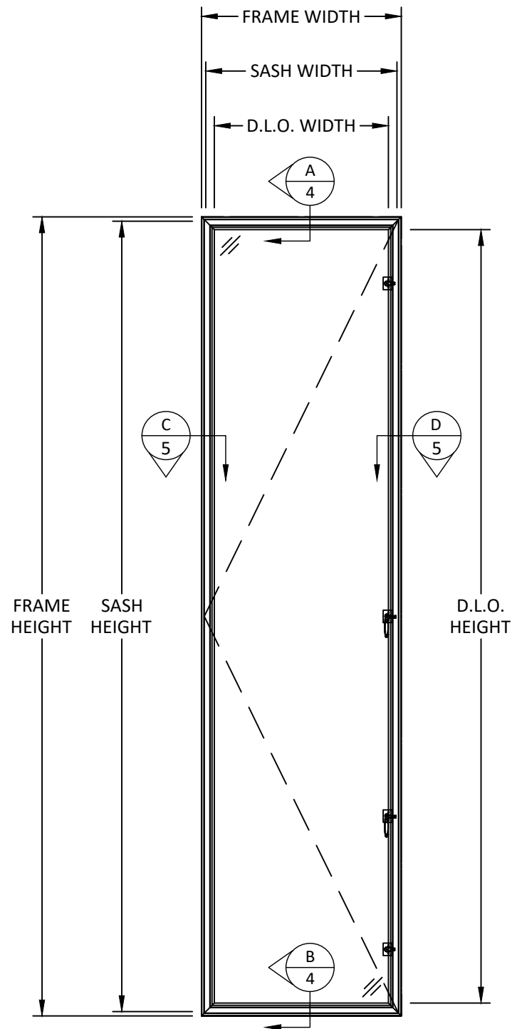
TYPICAL ELEVATION
