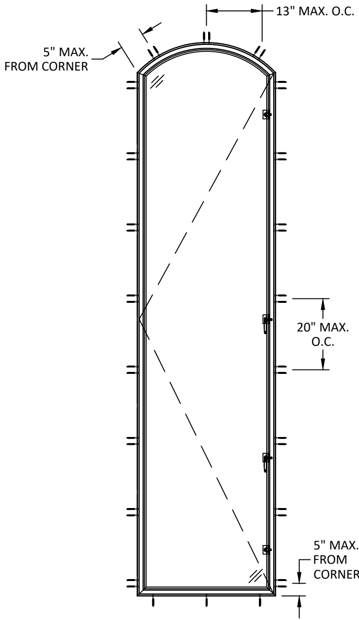
ANCHOR LAYOUT ARCH TOP
